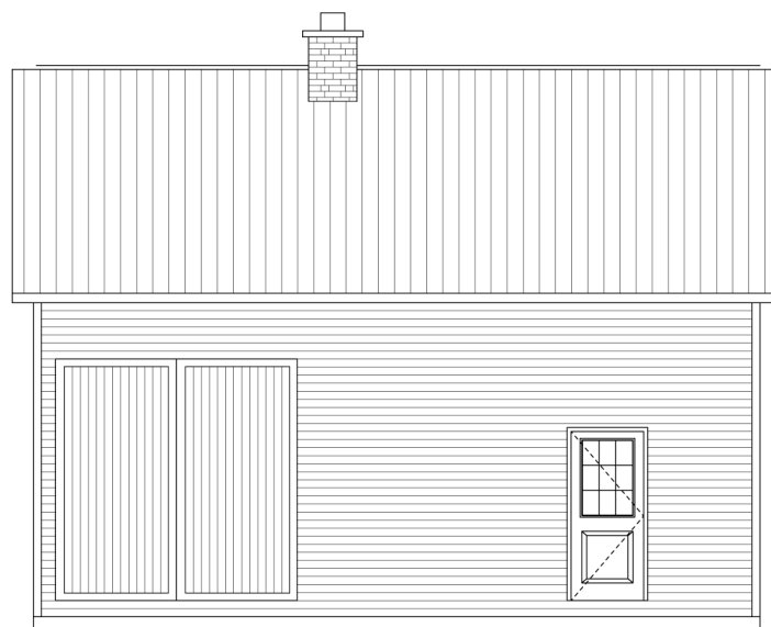
SOUTH ELEVATION
